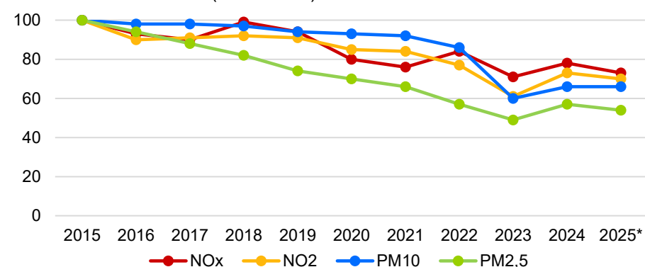
index verkeersemisseries (2015 = 100)
